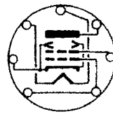
6P9
