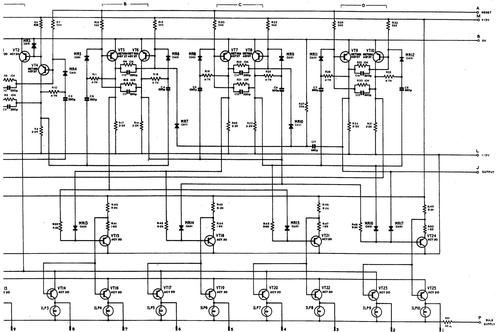
Circuit: Totalizer Type XG-S A.535
