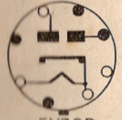
5Y3GB
