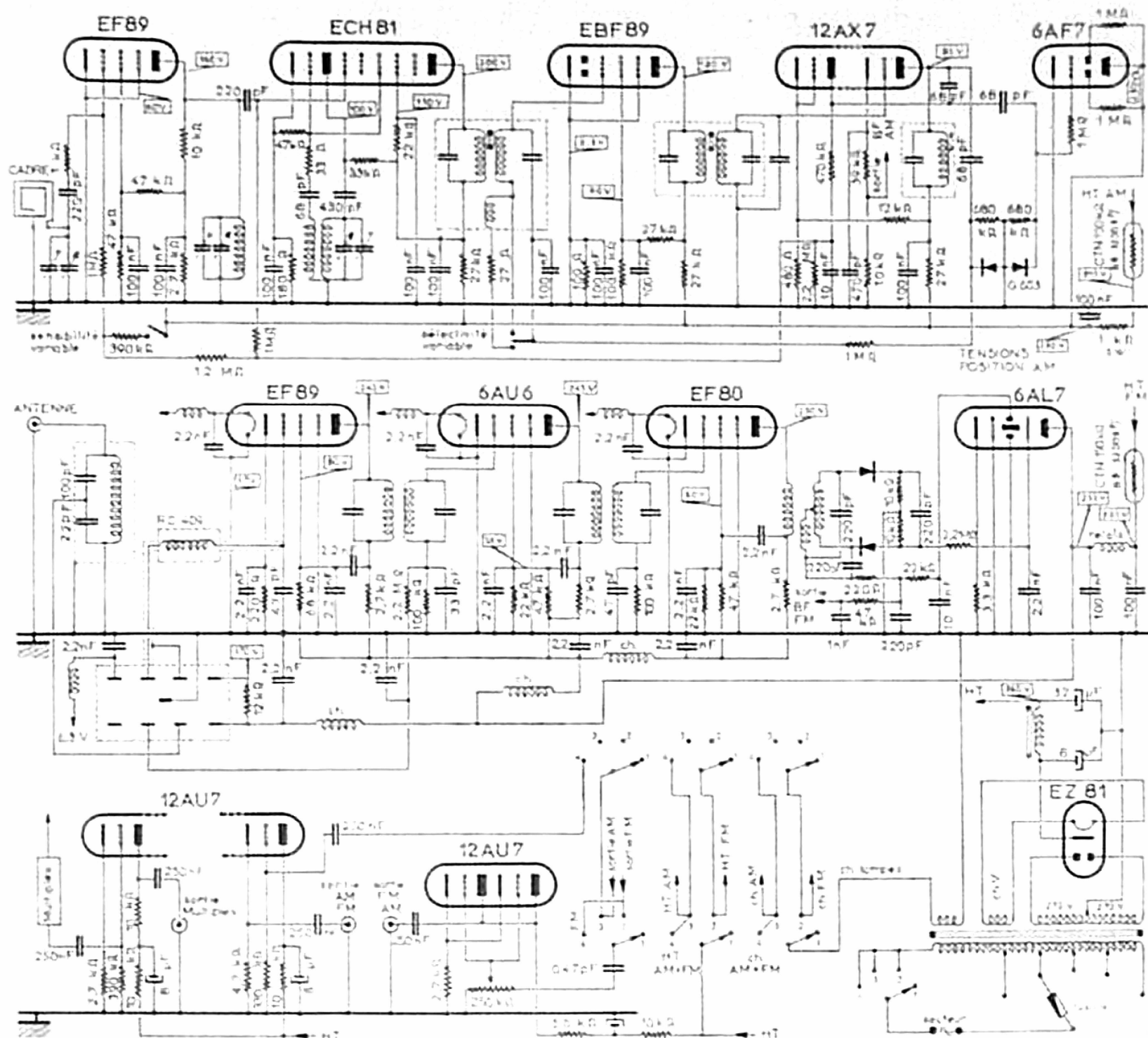
SCHEMA DU TUNER AM-FM ESART
