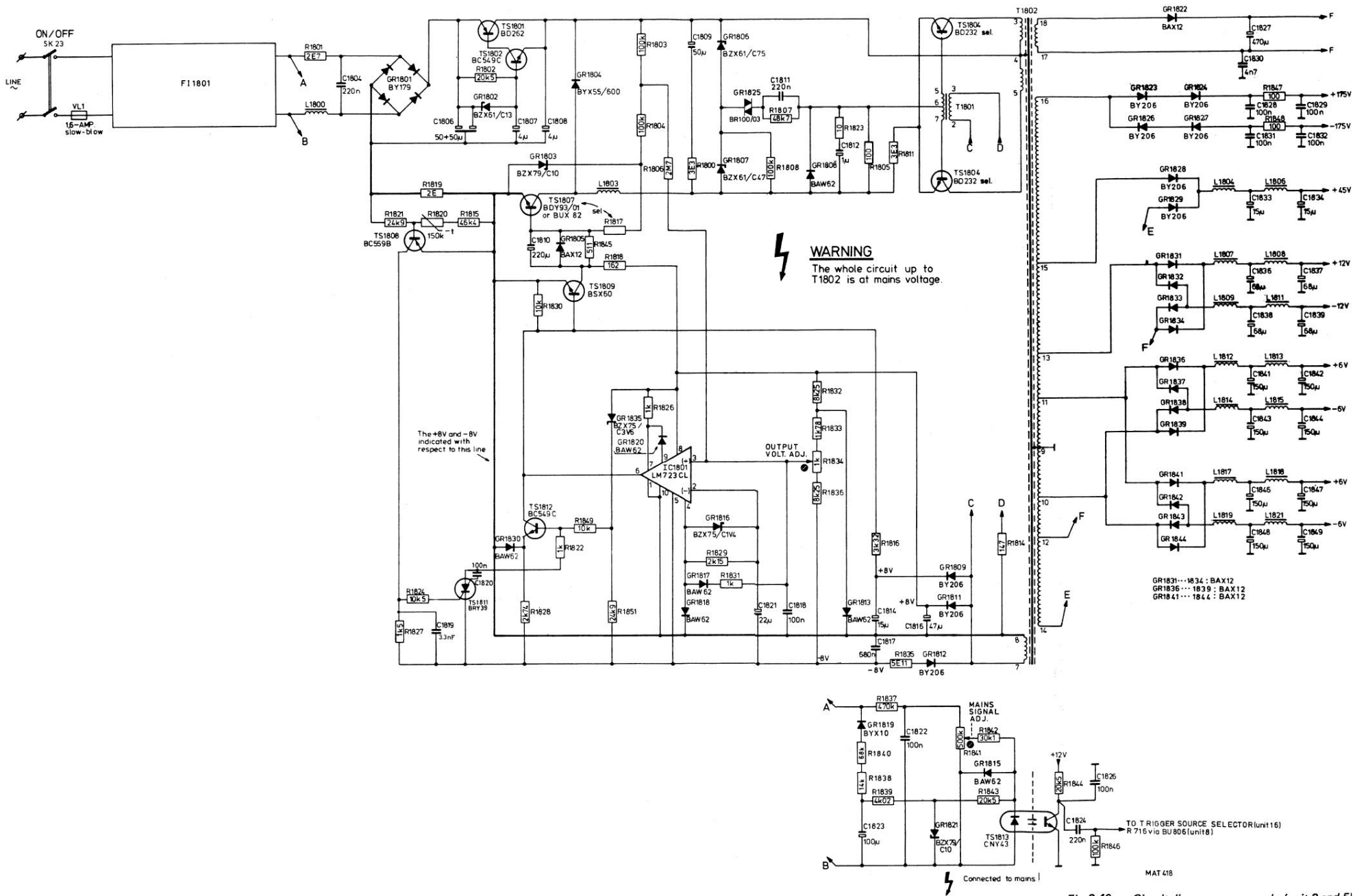
Fig. 3.40. Circuit diagram power supply (unit 3 and 5)
