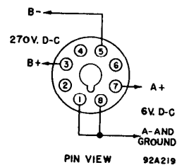
Fig. 2-1. Radio Receiver Model S-36A, wiring diagram for d-c power plug.
