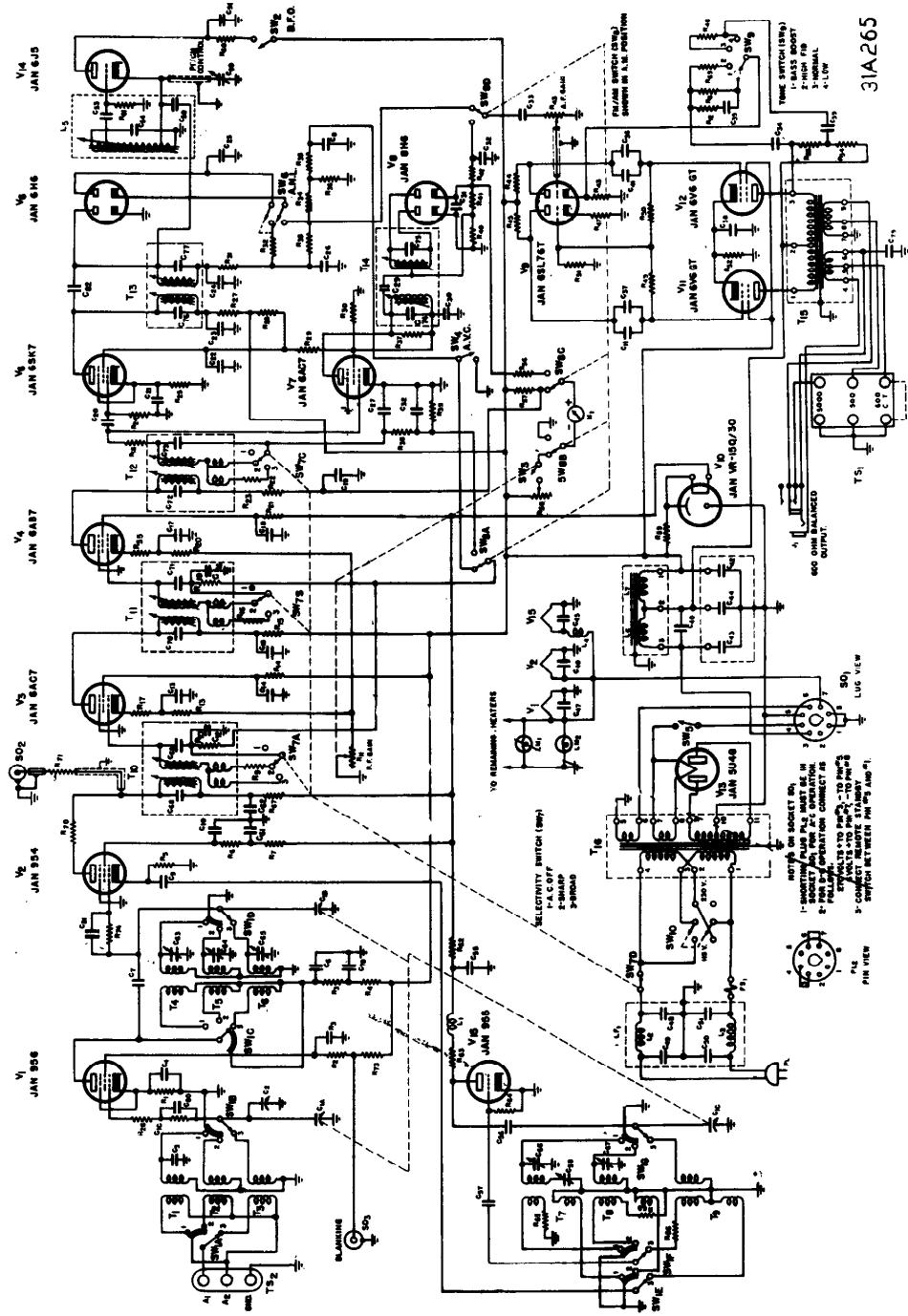
SCHEMATIC DIAGRAM-RADIO RECEIVER CHL-46131
