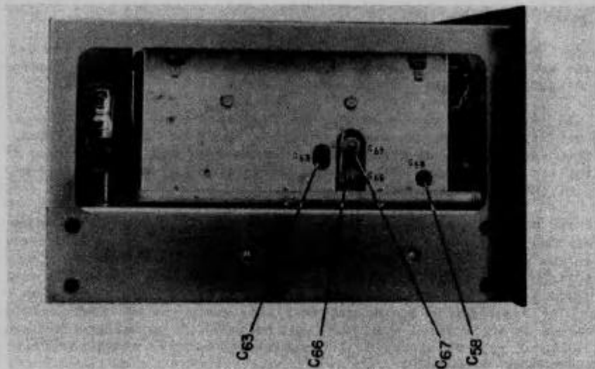
Figure 5-1. Radio Receiver Model S-36A, view showing alignment points.
